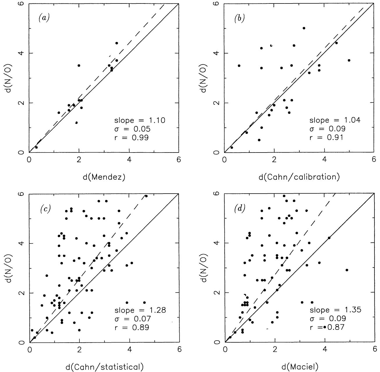
Fig. 1. Comparison of the N/O distances with (a) spectroscopic distances by Méndez et al. (1988; 1992); (b) calibration distances by Cahn et al. (1992); (c) statistical distances by Cahn et al. (1992), and (d) statistical distances by Maciel (1984).
