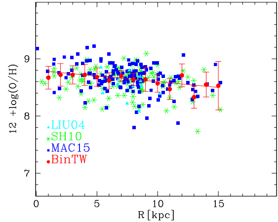
Figure 2. The radial distribution of the oxygen abundances, 12 + \log(O/H) , for PNe in the MWG. Data are from Liu et al. (2004), Stanghellini & Haywood (2010), and Maciel, Costa & Cavichia (2015), denoted by LIU04, SH10, and MAC15, respectively, as labelled in the legend. Our binned results are shown as red full dots with the least square straight line plotted over the points.
