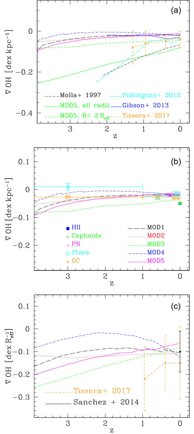
Figure 11. The evolution with redshift of the radial gradient of O abundances: (a) in dex \text{kpc}^{-1} units compared with cosmological simulations from Gibson et al. (2013) and Tissera et al. (2017), as labelled; (b) compared with observational data from different objects compiled in this work, as labelled; (c) in dex R_{\text{eff}}^{-1} units compared with cosmological simulations from Tissera et al. (2017) and data from Sánchez et al. (2014) and Sánchez-Menguiano et al. (2016a) for the present time. All panels show models MOD1–MOD5 with the same line coding as labelled in panel (b).
